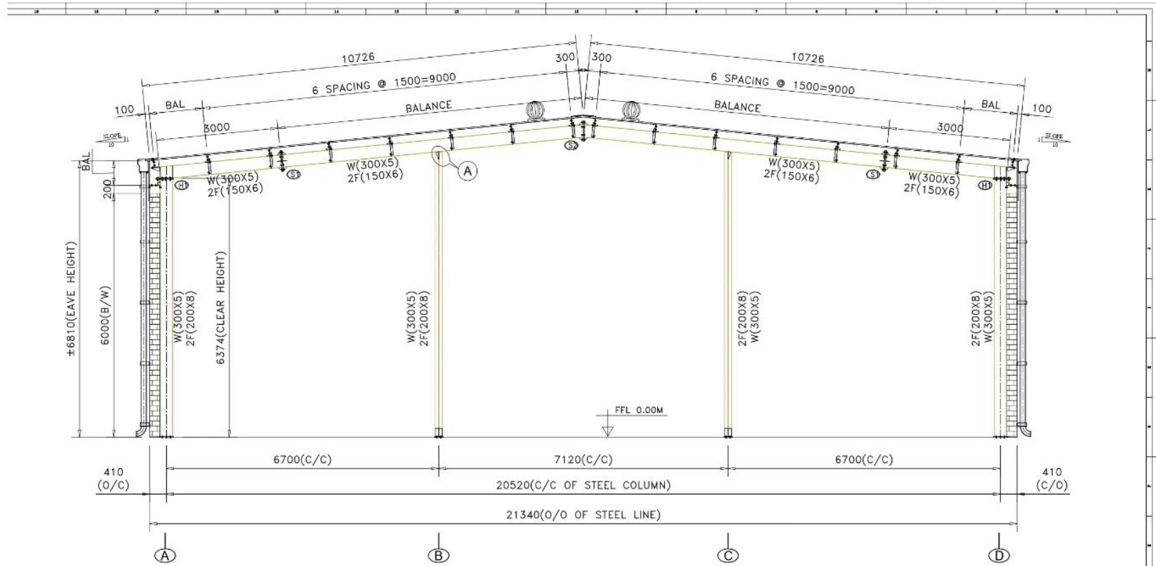
END FRAME ELEVATION @ F.L. :- 1 & 13 DOUBLE SIDED FLANGE BRACE
