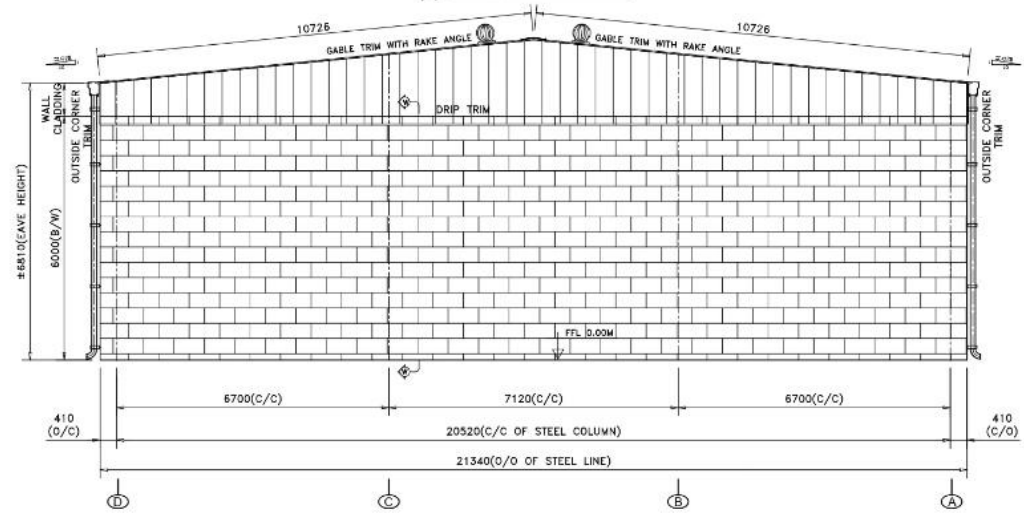
ENDWALL SHEETING ELEVATION : F. L- 13 PANEL WALL METAL SHEET (0.50 THK.) COLOUR. COLOUR COATED PANEL CUSTOMER TO CONFIRM WALL SHEETING & FLASHING COLOUR
