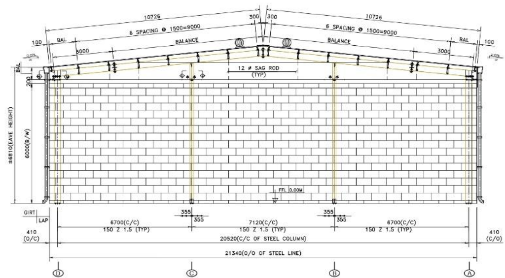
ENDWALL FRAMING ELEVATION @ F.L. :- 13 DOUBLE SIDED FLANGE BRACE
